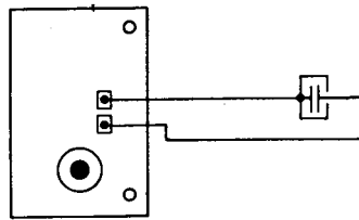
FIGURE 8. Recommended method of shielding auxiliary condenser.
